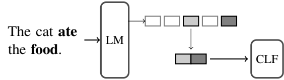
Figure 1: The figure illustrates the working principles of the classifiers developed by Yavas et al. (2023). The classifiers are trained to classify the relation between a predicate and its argument in a sentence using their contextualized word embeddings from a pre-trained language model as input.
