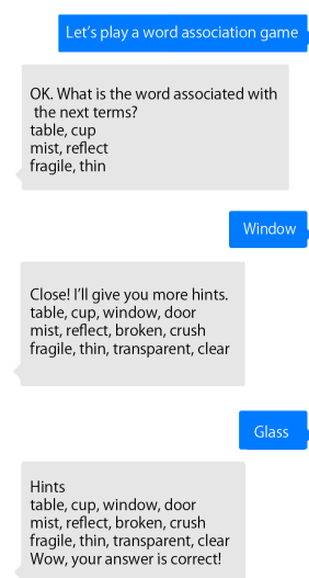
Figure 1: Word association game. Blue balloons show utterances of the player. All utterances of the player and the system are translated into English.
