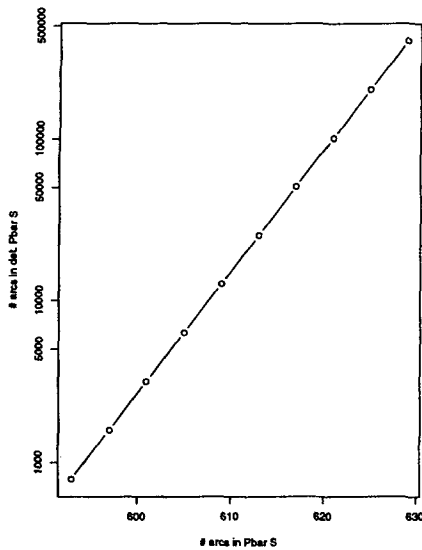
Figure 11: Number of arcs in the non-deterministic automaton \tau representing \overline{PS} = \overline{\Sigma_{>0}^* \rho_{>0} \Sigma_{>0}^*} versus the log of the number of arcs in the automaton obtained by determinization of \tau .
