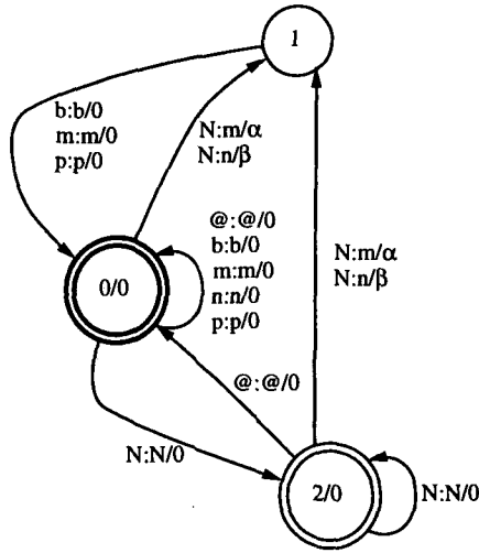
Figure 8: Transducer representing the rule 9.
