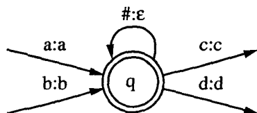
Figure 5: Filter transducer, TYPE 2.
