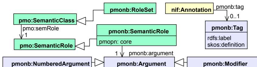
Figure 4: PreMON Ontology-NomBank module
