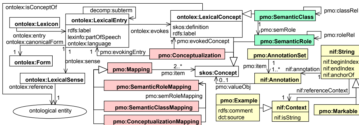
Figure 1: The PreMON Ontology extending lemon .
