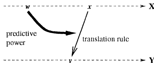
Figure 1: co-occurrence information
