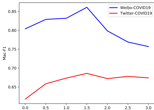
Figure 5: Effect of Adversarial Perturbation Norm \epsilon .
