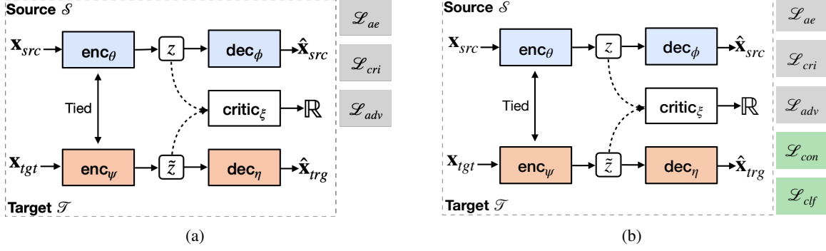
Figure 2: (a) \text{ARAE}_{seq2seq} – We replace the generator of \text{ARAE} with an encoder that encodes text from \mathcal{T} . (b) Adding our proposed cooperative losses to the model.
