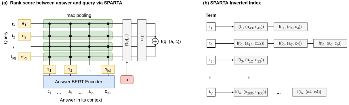
Figure 1: SPARTA Neural Ranker computes token-level matching score via dot product. Each query terms’ contribution is first obtained via max-pooling and then pass through ReLU and log. The final score is the summation of each query term contribution.
