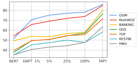
Figure 1: Masked LM prediction accuracy of BERT, DAPT with different data sizes, and TAPT models.
