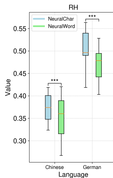
Figure 2: Box plots showing the RH scores from ten runs of the NeuralChar and NeuralWord models trained on the Chinese (Tong) and German (Leo) corpora from CHILDES. Statistical significance was determined by a paired permutation test at the sentence level (***: p < 0.001 ).
