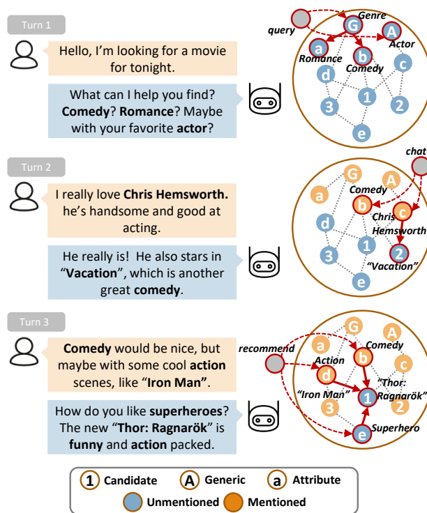
Figure 1: First three turns of an example dialog. The dialog is shown on the left with entities on the KG in bold. The graph on each dialog turn's right demonstrates the reasoning process of CR-Walker, with the reasoning tree marked red. Throughout this paper, candidate items are noted with numbers, and generic classes / attributes with upper-/lower-case letters. The orange/blue color indicates that the entity is mentioned/unmentioned in the previous context.
