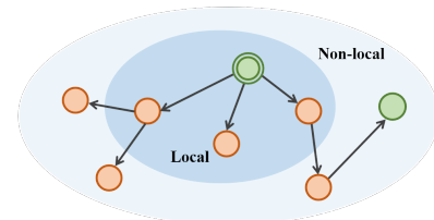
Figure 1: Two limitations if edge features are retrieved from a fixed-size embedding matrix: (a) fail to discover useful meta-paths, and (b) unable to differentiate local and non-local neighbors.
