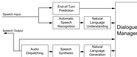
Figure 1: Schematic of an incremental spoken dialogue network containing parts for speech understanding and end-of-turn prediction on the top, the dialogue managing unit on the right and the speech generation and audio dispatching on the bottom.
