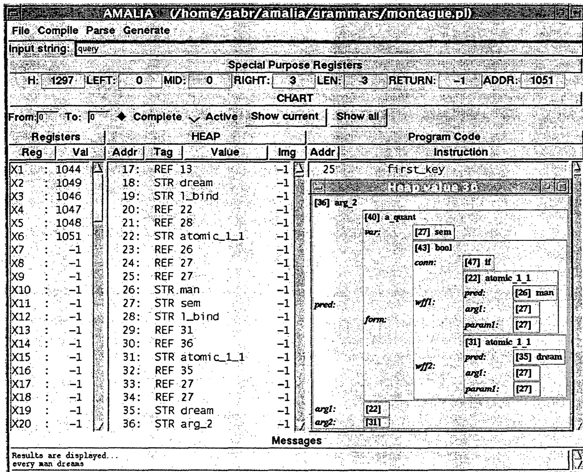
Figure 2: A sample screen shot of AMALIA.
