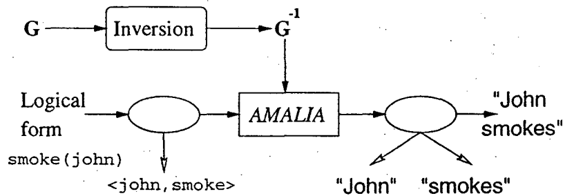
Figure 1: An overview of generation with Abstract Machine.
