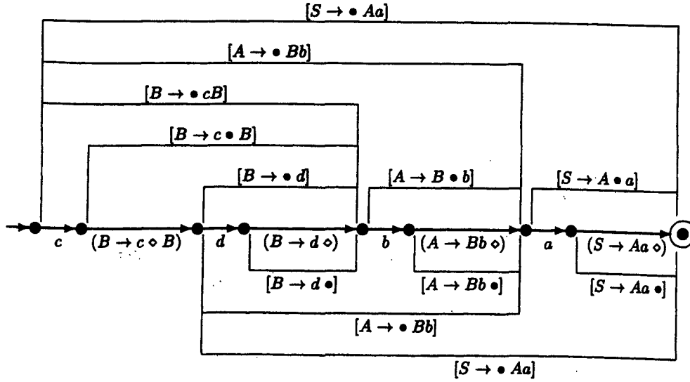
Figure 4. A finite automaton resulting from simulating the transducer on input cdba (thick lines), and the subsequent table U of dotted items (thin lines).
