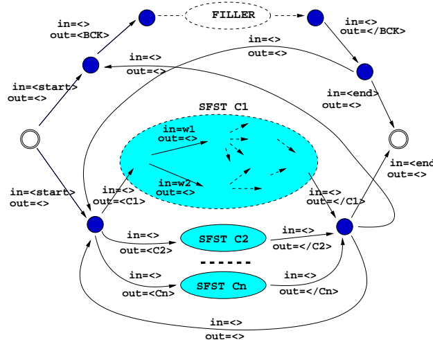
Figure 1: Word-to-Concept Transducer
