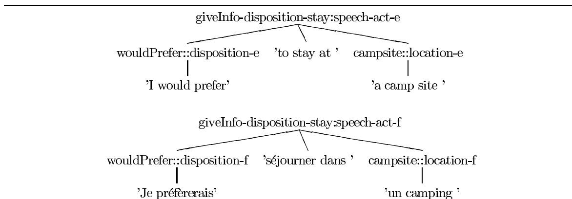
Figure 2: Abstract typed trees in English and French for the sentence I would prefer to stay at a camp site
