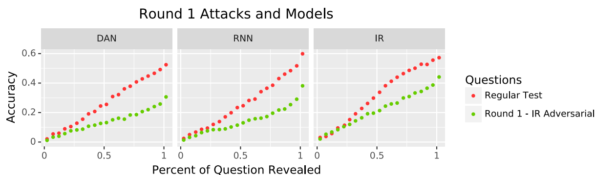
Figure 4: The first round of adversarial writing attacks the IR model. Like regular test questions, adversarially-authored questions begin with difficult clues that trick the model. However, the adversarial questions are significantly harder during the crucial middle third of the question.
