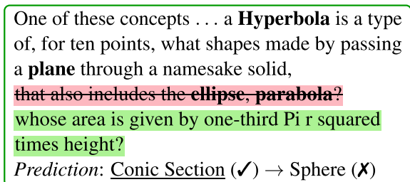
Figure 8: The interpretation successfully aids an attack against the IR system. The author removes the phrase containing the words “ellipse” and “parabola”, which are highlighted in the interface (shown in bold ). In its place, they add a phrase which the model associates with the answer sphere .
