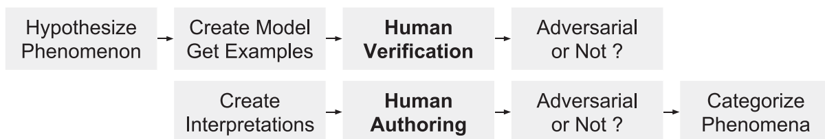
Figure 1: Adversarial evaluation in NLP typically focuses on a specific phenomenon (e.g., word replacements) and then generates the corresponding examples (top). Consequently, adversarial examples are limited to the diversity of what the underlying generative model or perturbation rule can produce—and also require downstream human evaluation to ensure validity. Our setup (bottom) instead has human-authored examples, using human–computer collaboration to craft adversarial examples with greater diversity.
