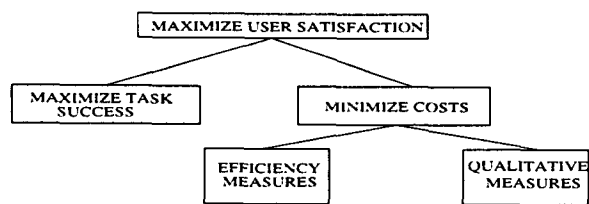
Figure 5: PARADISE's structure of objectives for spoken dialogue performance.
