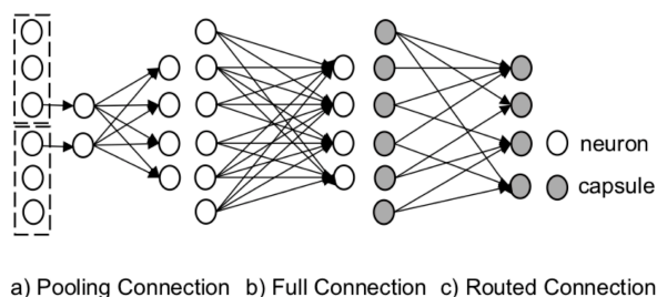
Figure 2: Outputs attend to a) active neurons found by pooling operations b) all neurons c) relevant capsules found in routing processes.
