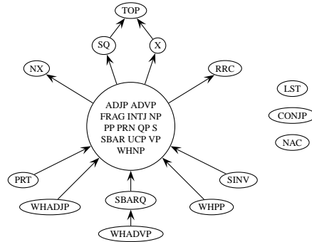
Figure 7: The same-span-reachability graph for the NOEMPTIES grammar.
