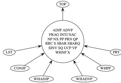
Figure 6: The same-span reachability graph for the NOTTRANSFORM grammar.
