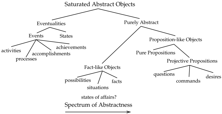
Figure 1 Asher’s typology of saturated abstract objects (Asher 1993, page 57).
