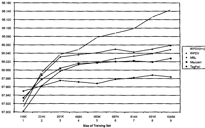
Figure 5 The accuracy of combiner methods on LOB as a function of the number of tokens of training material.
