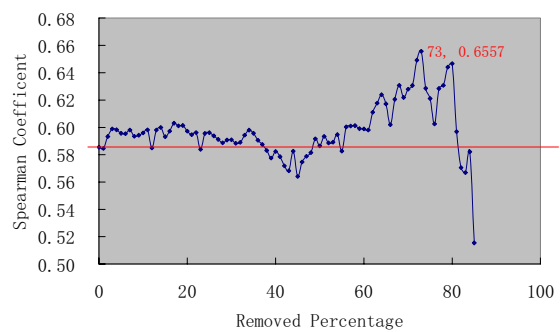
Figure 4. Spearman Coefficient of ASSBC vs. different percentage of removed systems on TREC -7.
