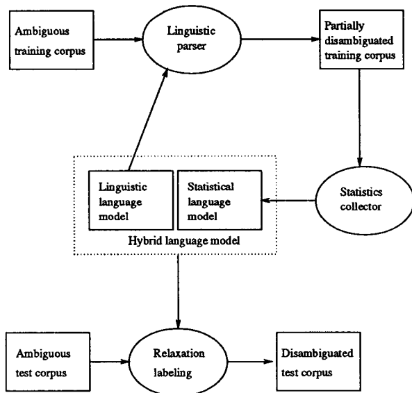
Figure 1: Parser architecture.
