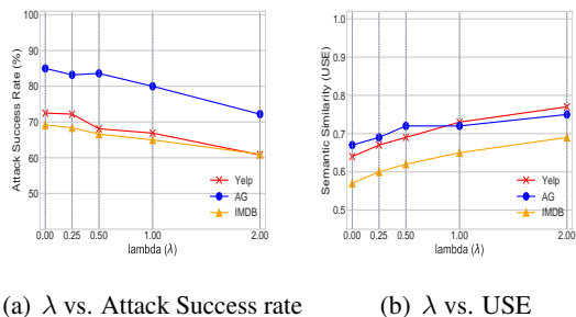
Figure 2: Effect of the semantic similarity constraint on S2B2-Attack’s performance. The classifier is Roberta.
