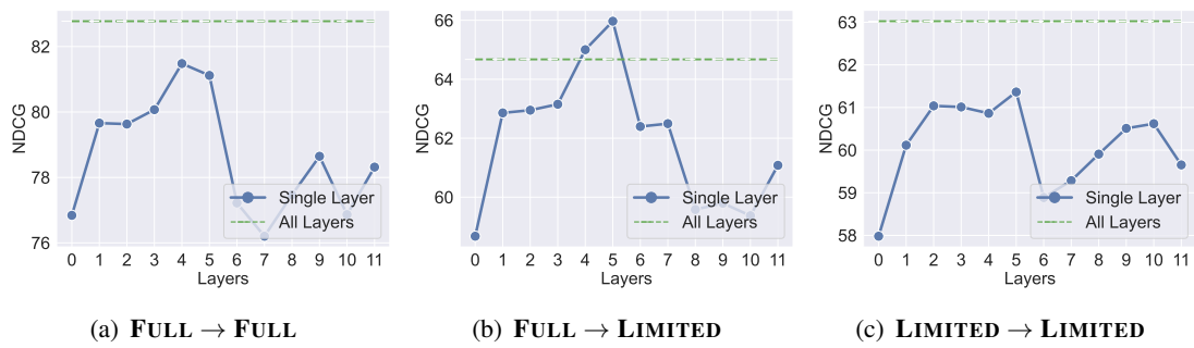
Figure 10: The impact of using one single transformer layer for embedding generation. The NDCG is an average of different transfer settings.
