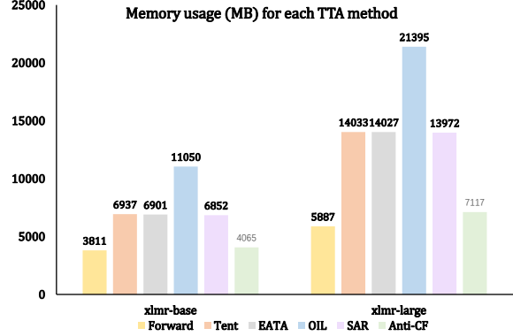
Figure 7: Memory usage of various TTA methods.
