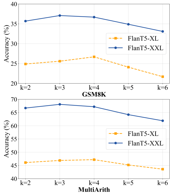
Figure 6: The effect of hyperparameter k on the model performance on the GSM8K and MultiArith datasets.
