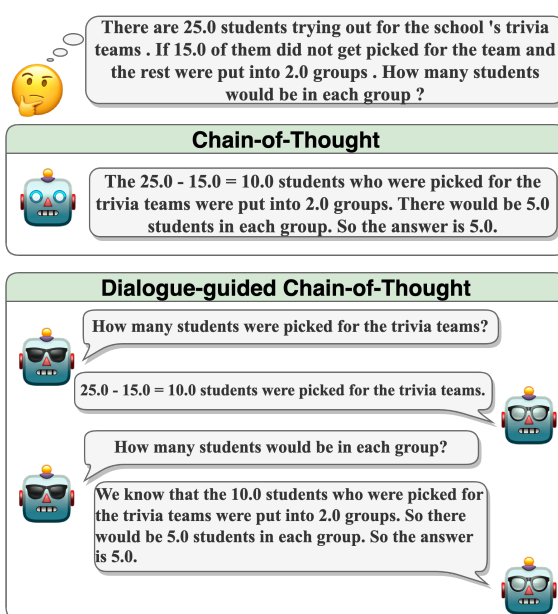
Figure 1: A comparison of DialCoT and CoT prompting (Wei et al., 2022). CoT prompting guides the model to output all intermediate reasoning steps at once to obtain the final answer, while DialCoT leads the model to gradually generate intermediate reasoning steps in a dialogic format to ultimately arrive at the answer.
