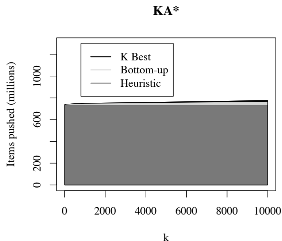
Figure 4: The performance of \text{KA}^* for lexicalized grammars. The performance is dominated by the computation of the heuristic, so that both the bottom-up phase and the k -best phase are barely visible.
