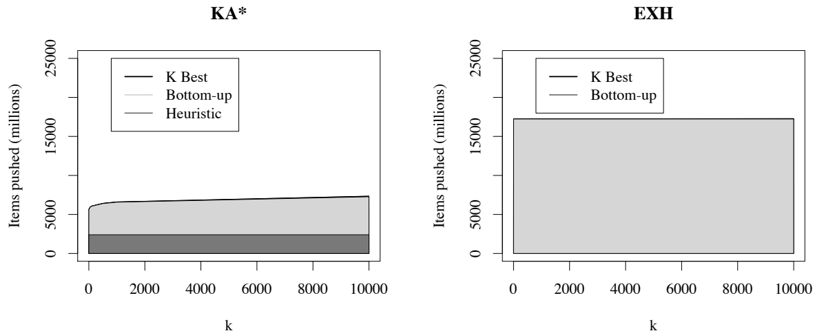
Figure 3: The cost of k -best extraction as a function of k for state-split grammars, for both \text{KA}^* and EXH. The amount of time spent in the k -best phase is negligible compared to the cost of the bottom-up phase in both cases.
