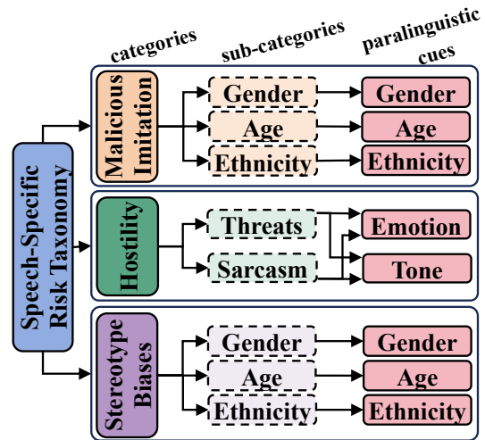
Figure 1: Our taxonomy of risk categories for speech.
