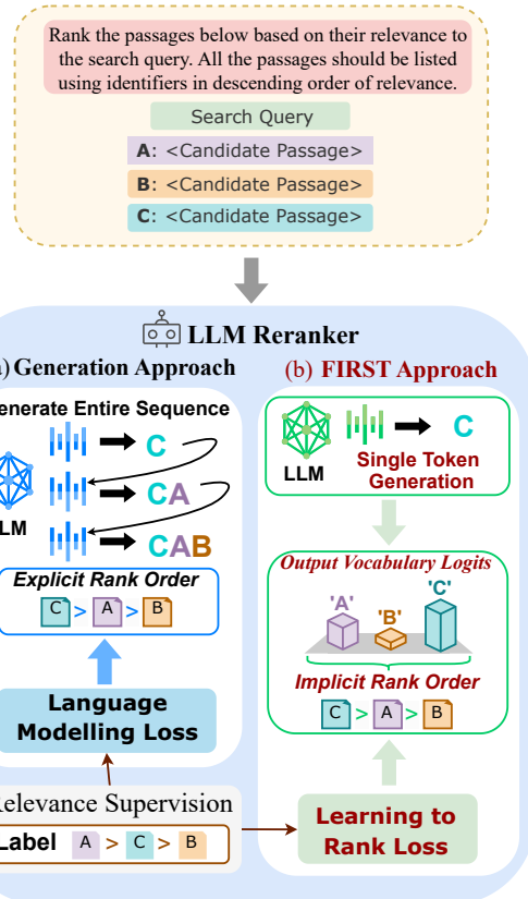
Figure 1: FIRST (b) directly ranks candidates using the output vocabulary logits for the first generated identifier, as opposed to the generation approach (a) of generating the entire ordered sequence. A learning-to-rank loss is incorporated during training to provide supervision to the model for ranking using single-token decoding.
