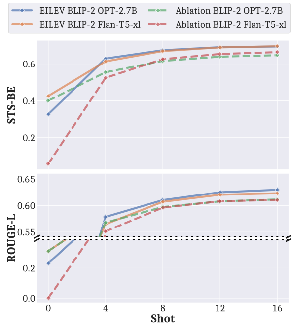
Figure 8: Results for the dynamic meaning ablation experiment.
