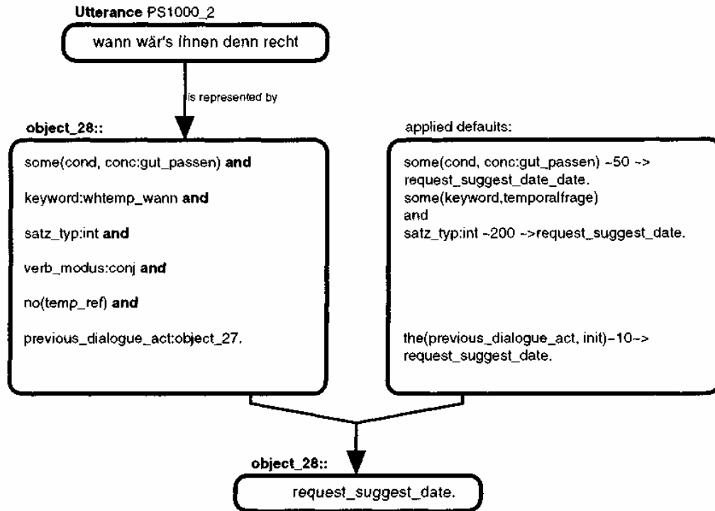
Figure 3: Determining the dialogue act for utterance (8).
