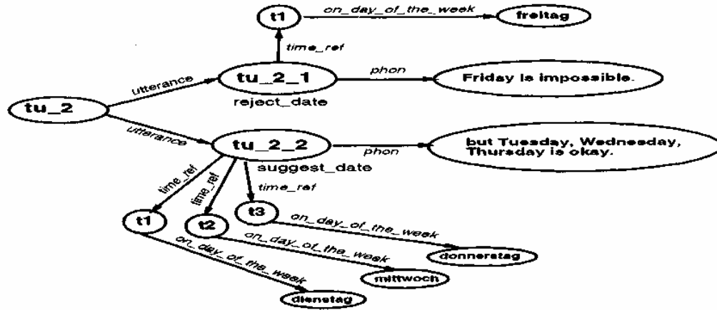
Figure 2: The FLEX representation of the interpreted utterance.
