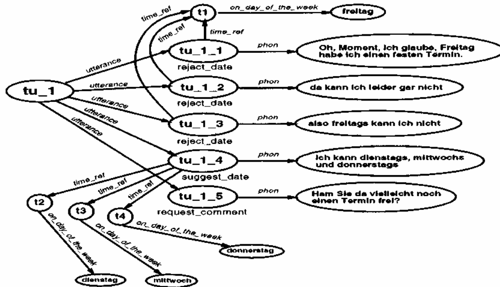
Figure 1: The FLEX representation of the source-language utterance.
