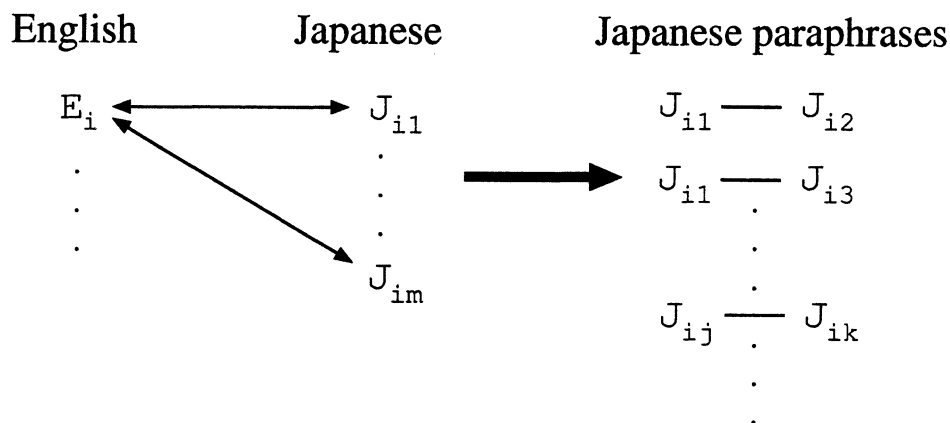
Figure 1: Extracting Paraphrases
