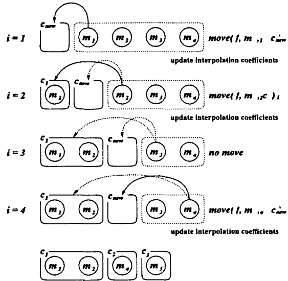
Figure 2: The clustering algorithm.
