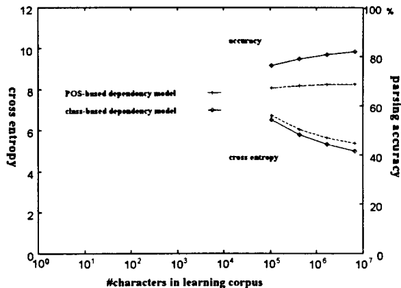
Figure 3: Relation between cross entropy and parsing accuracy.
