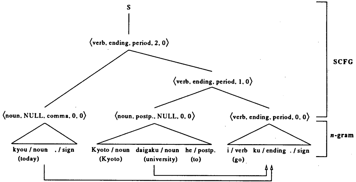
Figure 1: Dependency model based on bunsetsu
