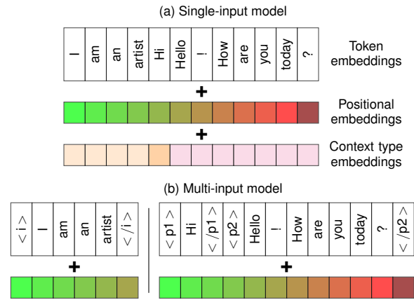
Figure 2: Token embeddings: (a) single-input model with CTE; (b) multi-input model with start/end tokens.
