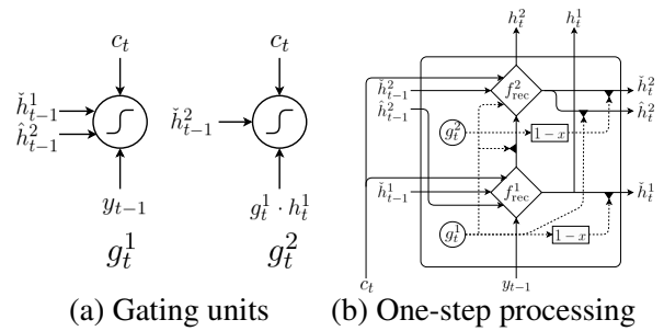
Figure 1: Bi-scale recurrent neural network
