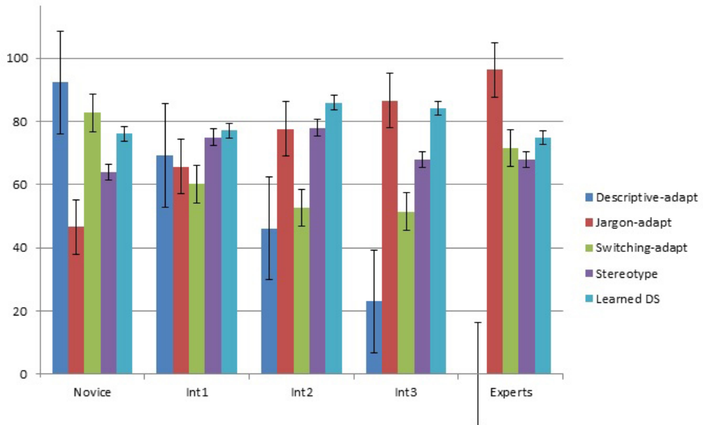
Figure 7 Evaluation: Adaptation Accuracy vs. User types.
