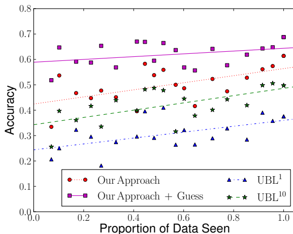
Figure 4: Meaning Prediction: Train on files 1, \dots, n test on file n + 1 .
