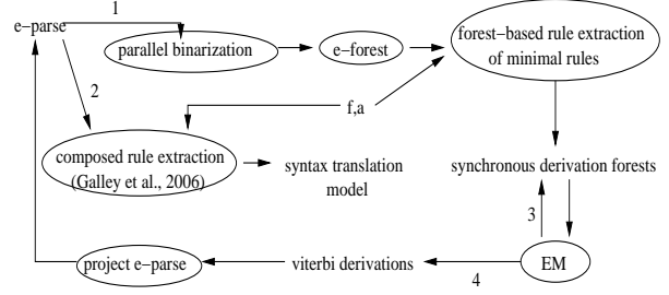
Figure 5: Using the EM algorithm to choose restructuring.
