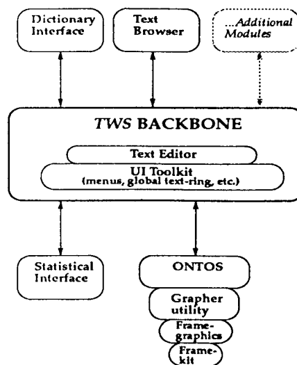
Figure 1: TWS architecture. The system was designed to make it easy to plug new modules into TWS.
