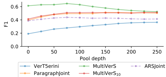
(b) F1 score as a function of pool depth. The blue dot at pool depth 100 indicates that VERT5ERINI would have achieved an F1 score of roughly 30, if annotation had stopped at a depth of 100. Results are ARSJOINT are shown as a dashed line to indicate that this system was not used for data collection.
