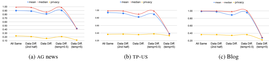
Figure 2: The correlation between the empirical privacy of AIA and the maximum posterior probability. mean and median denote the mean and median of the maximum posterior probability of the queries.
