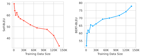
Figure 5: Test set performance of model fine-tuned on varying amount of data in MULTIPIT AUTO , in terms of Self-BLEU (lower is better) and BERT-iBLEU.
