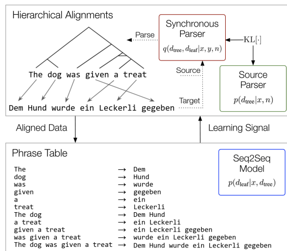
Figure 1: An overview of our approach. During training a variational synchronous parser hierarchically segments and aligns source-target phrases (top), which provides training pairs for a seq2seq model (bottom). The seq2seq loss provides learning signal to the synchronous parser which subsequently provides signal to (and is regularized by) a monolingual source parser. After training, there are two inference models: one mode in which both parsers are discarded, which results in a regular seq2seq model that has been regularized by latent hierarchical phrase pairs; another mode in which the seq2seq model can be combined with the source parser to derive a neural synchronous grammar. Inference in this mode is done via translation-as-parsing with cube-pruned CKY.
