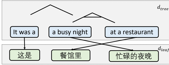
Figure 3: Induced hierarchical alignment by BTG-Seq2Seq on an English-Chinese example.
