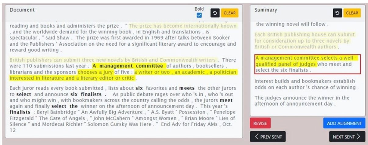
Figure 2: The Highlighting Annotation UI, presenting a document and its corresponding summary. Saved alignments have a faded yellow background, whereas currently selected alignments (which haven't been saved yet) have a normal yellow background. The current summary sentence is marked in a red box. Also, the bold feature is activated, meaning the document words which are related to those in the summary sentence are boldfaced (see §4.1).
