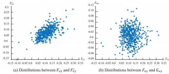
Figure 5: Joint distributions of encoder features between (a) RLM ( F_{<t} ) and HLM ( F_{<t}^* ), (b) RLM ( F_{<t} ) and HLM with subtracting LM ( G_{<t} ). (a) shows correlations with F_{<t}^* by grammatical knowledge in HLM, and (b) shows relatively independent distributions by G_{<t} .
