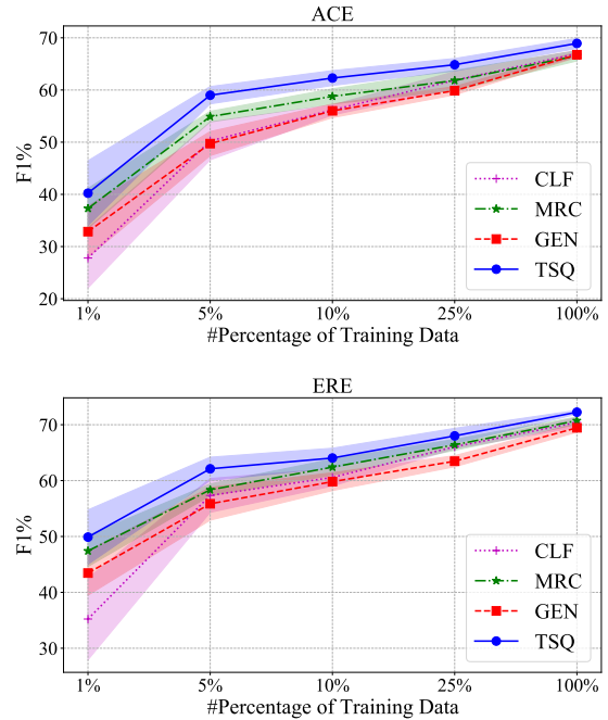
Figure 5: Argument F1(%) scores on ACE and ERE test sets with different amounts of training data. Here x -axis (drawn in log scale) denotes the percentage of original training data sampled. The shaded areas indicate the ranges of standard deviations.
