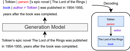
Figure 6: Label-augmented Sequence.
