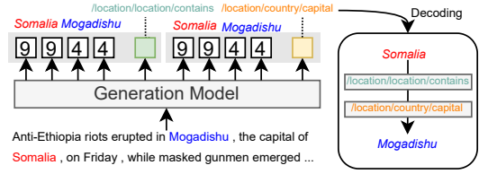
Figure 7: Indice-based Sequence.
